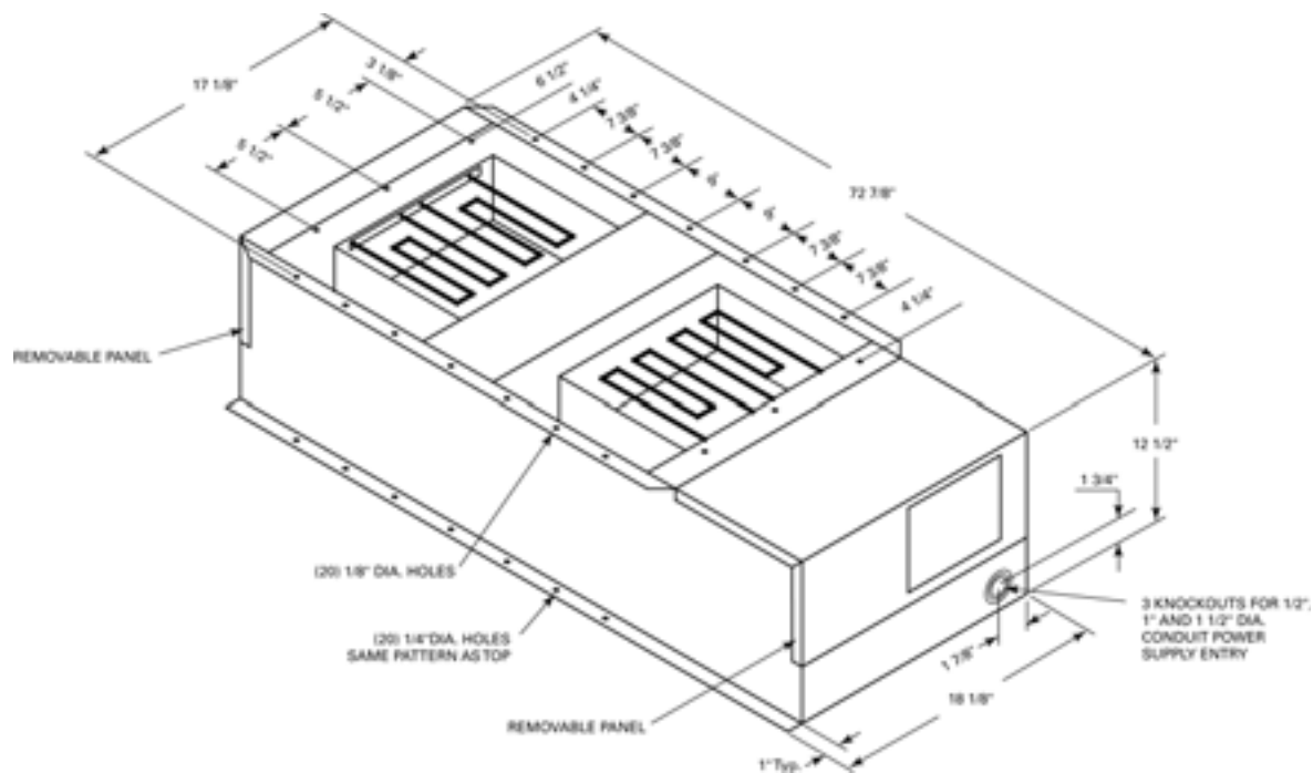
Figure 40. Electric Heater Accessory for over 10 Ton Air Handlers. All dimensions are in inches.
