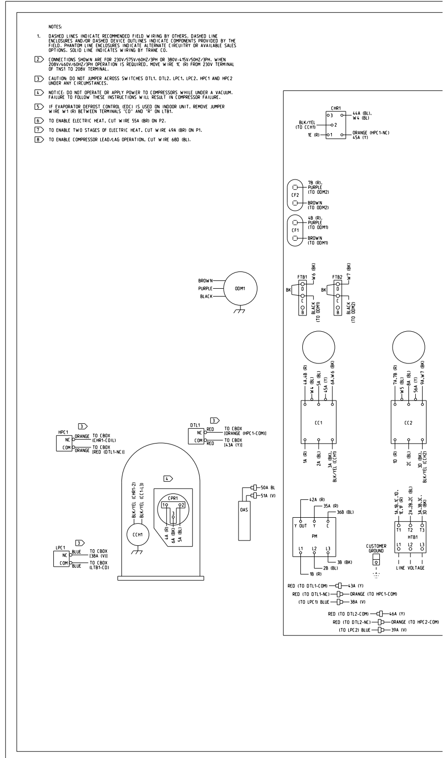
Figure 19. Typical Dual Compressor - Connection Diagram
