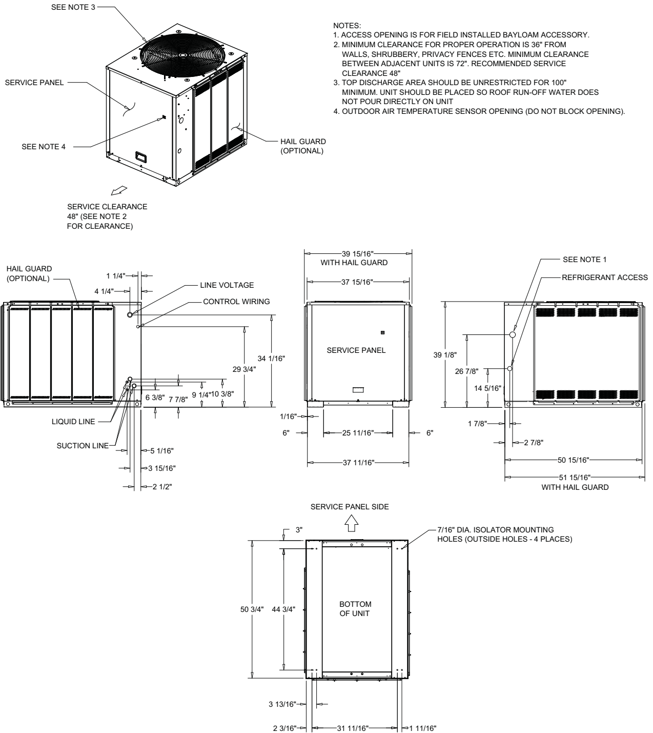
Figure 24. 10 Ton Condensing Unit, Dual Compressor
