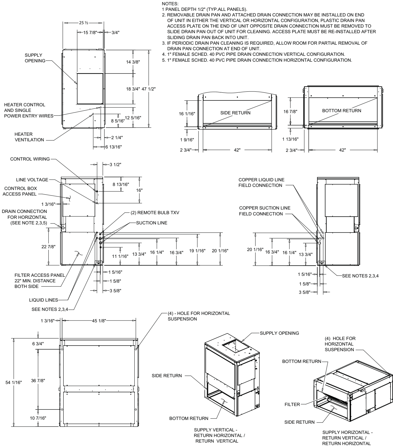
Figure 32. 7 1/2 Ton Air Handler, Dual Circuit
