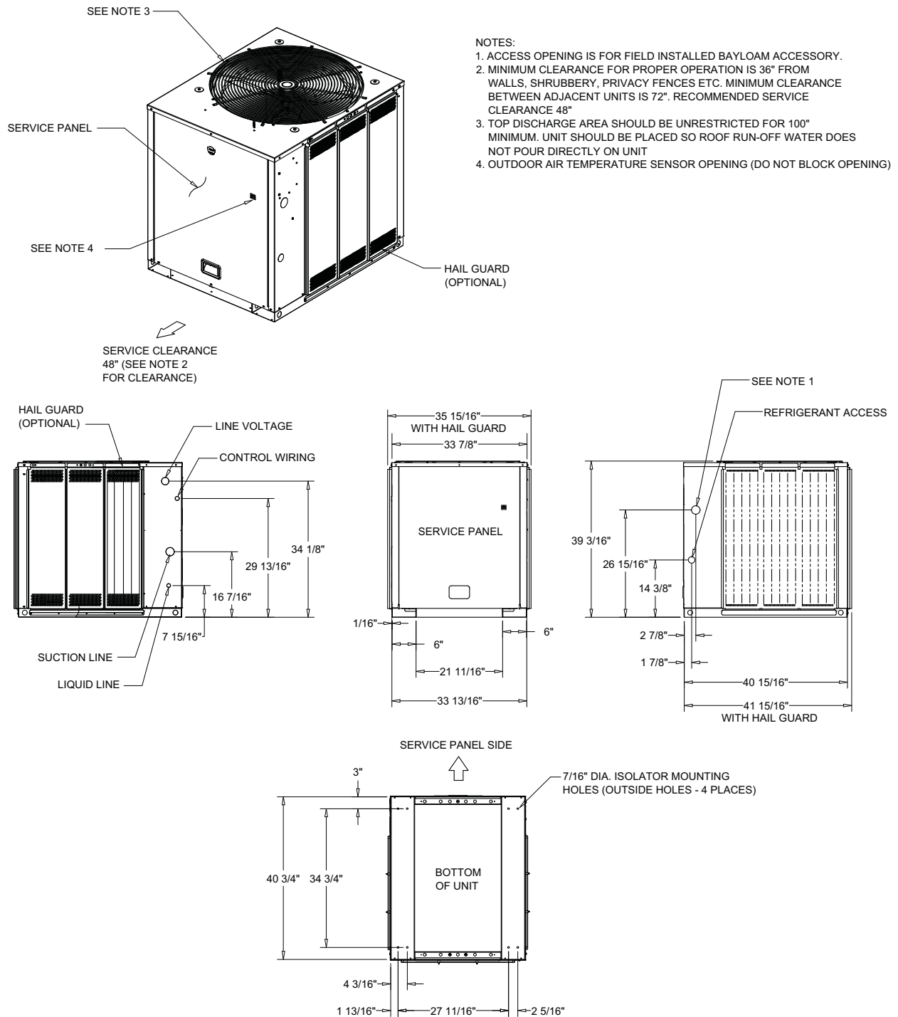
Figure 22. 6-7 1/2 Ton Condensing Unit, Single Compressor
