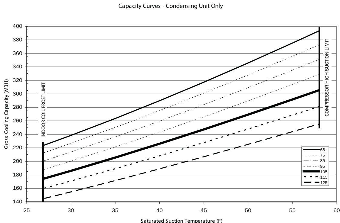
Figure 16. TTA240F - Both Compressors - Capacity Curves
