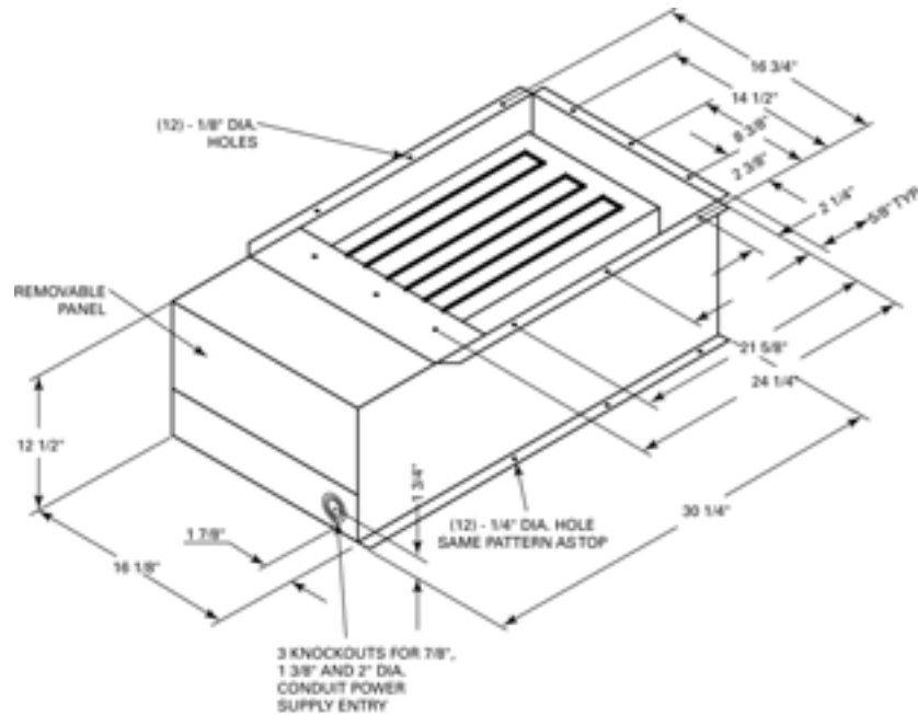
Figure 39. Electric Heater Accessory for 10 Ton and Under Air Handlers. All dimensions are in inches.
