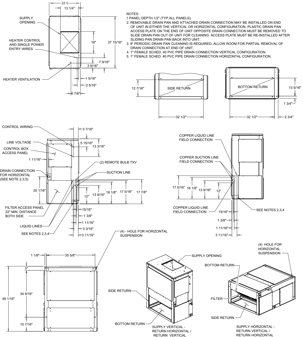
Figure 30. 5 Ton Air Handler, Dual Circuit
