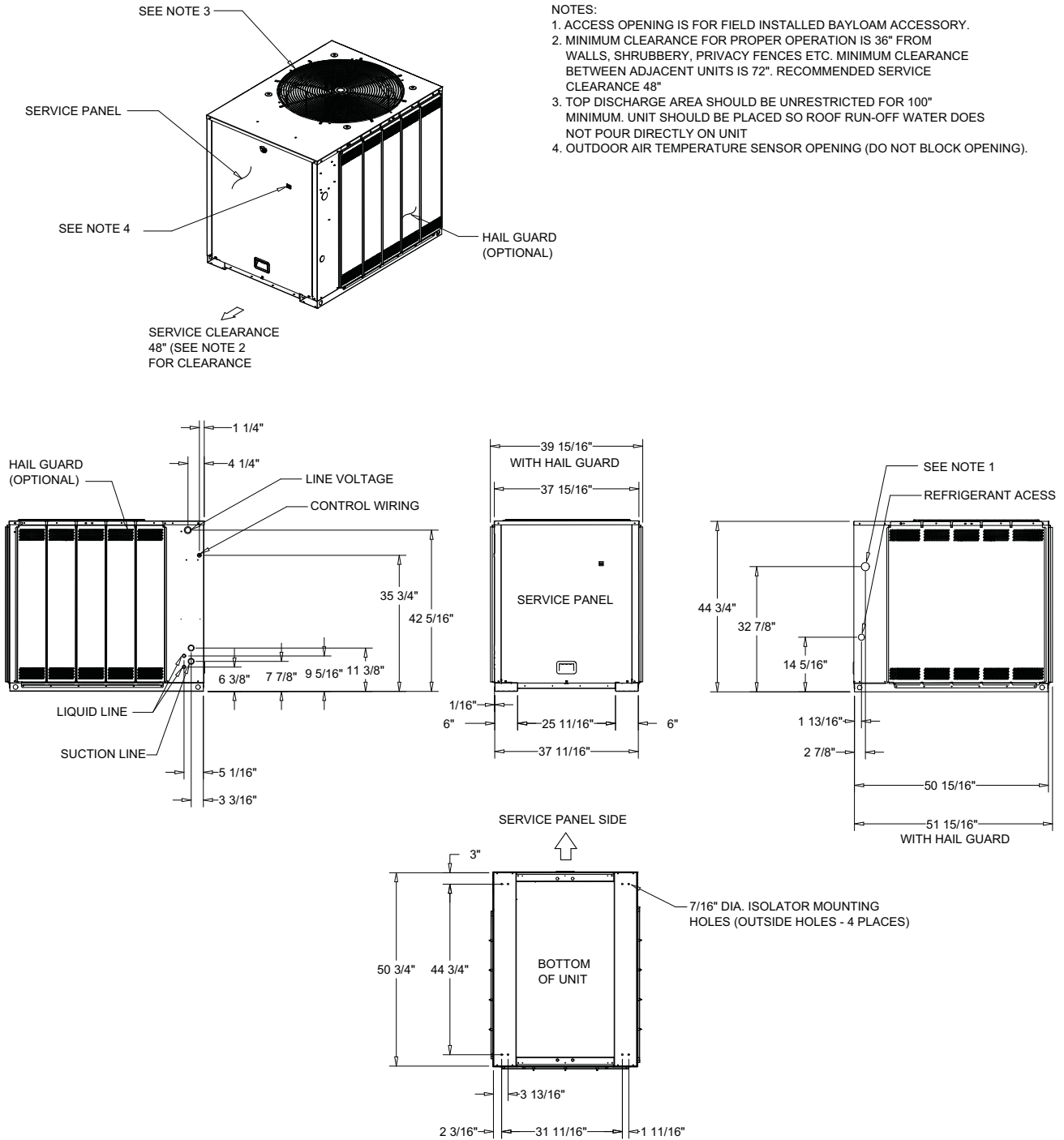
Figure 26. 12 Ton Condensing Unit, Dual Compressor
