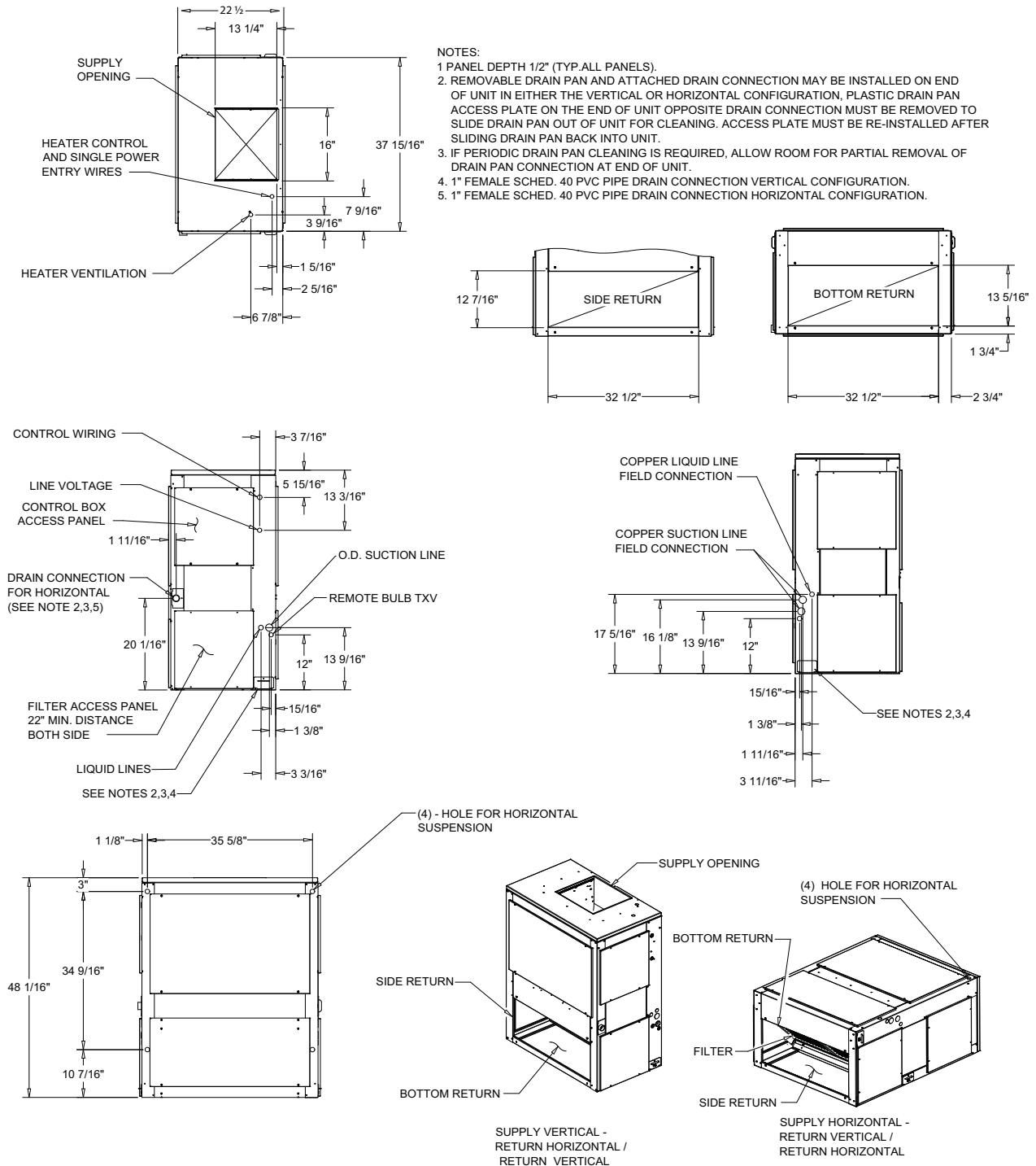
Figure 29. 5 Ton Air Handler, Single Circuit
